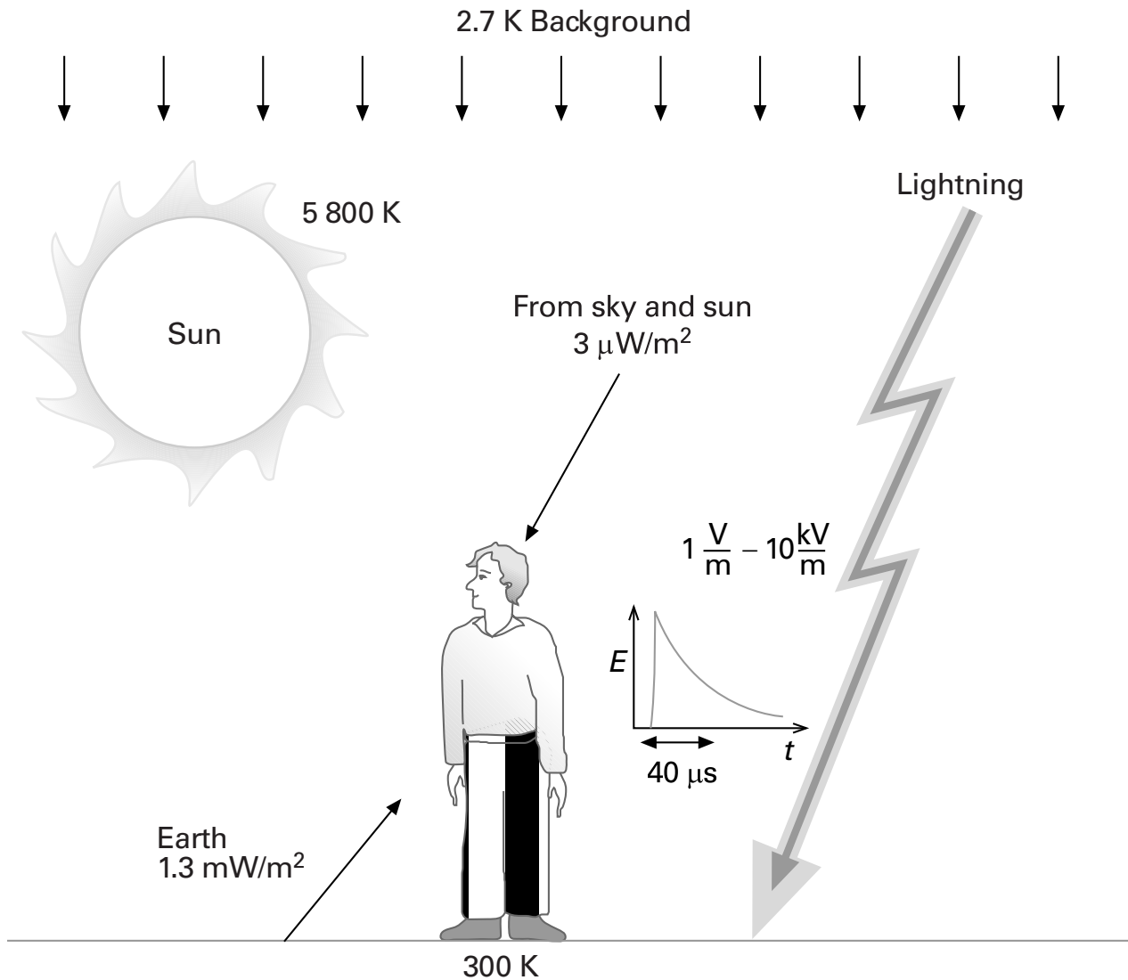
Fig. 1.3 Terrestrial and extraterrestrial sources of radiofrequency radiation
